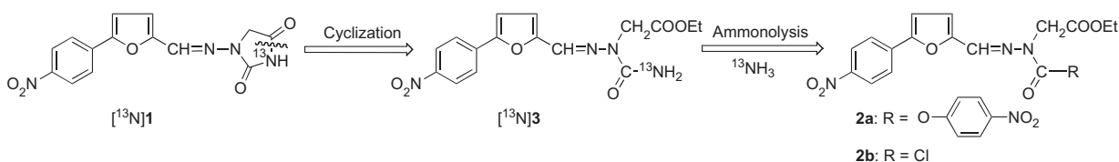
Scheme 2. Retrosynthesis of ^{13}\text{N} 1 .
