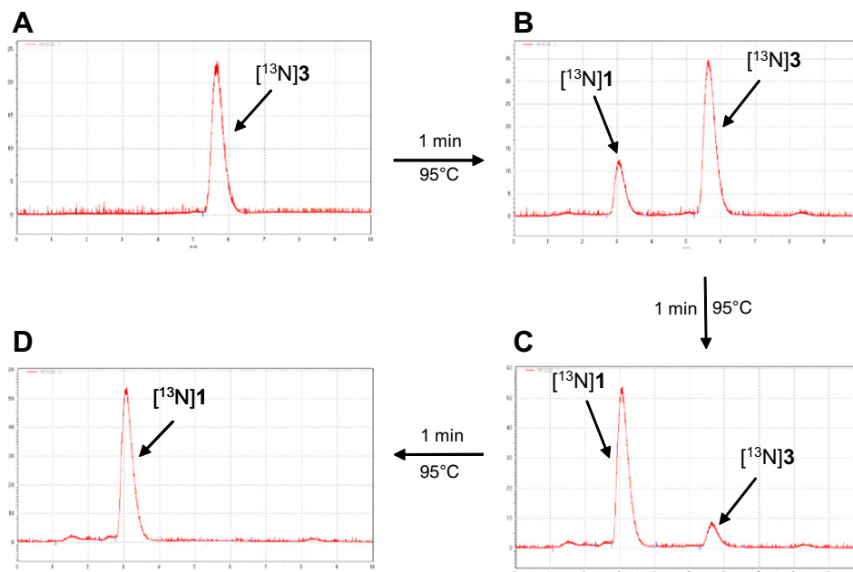
Figure 1. HPLC analytical chromatograms reflecting the cyclization process of [ ^{13}\text{N} ]3 (retention time: 5.5 min) to form [ ^{13}\text{N} ]1 (retention time: 3.1 min) in \text{CH}_3\text{CN} and \text{H}_2\text{O} at 95^\circ\text{C} : (a) before heating the HPLC fraction containing [ ^{13}\text{N} ]3; (b) heating [ ^{13}\text{N} ]3 for 1 min; (c) heating [ ^{13}\text{N} ]3 for 2 min; (d) heating [ ^{13}\text{N} ]3 for 3 min. The analytical conditions were as follows: Shiseido Capcell Pak \text{C}_{18} (4.6 mm \phi \times 250 mm), \text{H}_2\text{O}/\text{CH}_3\text{CN} (6/4), 1.0 mL/min, 254 nm. The identity of [ ^{13}\text{N} ]3 or [ ^{13}\text{N} ]1 was confirmed by co-injection with the non-radioactive 3 or 1.
