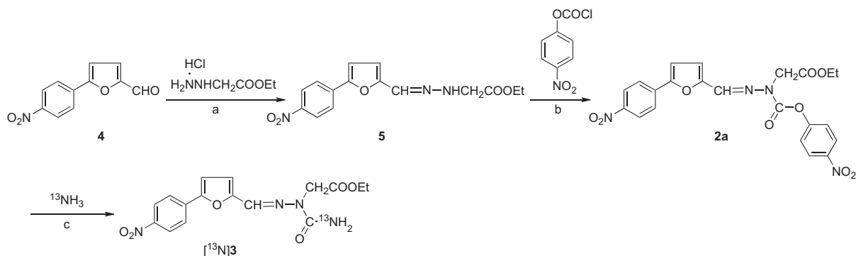
Scheme 3. Chemical synthesis and ^{13}\text{N} ammonolysis of 2a . Reagents and conditions: (a) DMF, \text{H}_2\text{O} , room temperature, 24 h, 69%; (b) \text{Et}_3\text{N} , \text{CH}_2\text{Cl}_2 , room temperature, 12 h, 64%; (c) base ( \text{K}_2\text{CO}_3 , pyridine, \text{Et}_3\text{N} , DMAP, i\text{-Pr}_2\text{NEt} or lutidine), solvent (THF, DCE, \text{CH}_3\text{CN} or DMF), 75^\circ\text{C} , 3 min, 2–60%.
