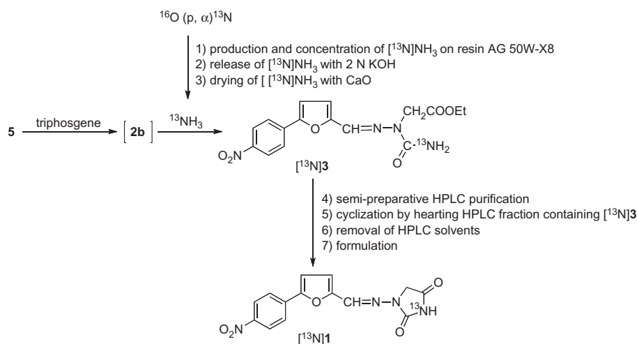
Scheme 5. Automated synthesis of [ ^{13}\text{N} ]1 using no-carrier-added [ ^{13}\text{N} ]NH _3 .
