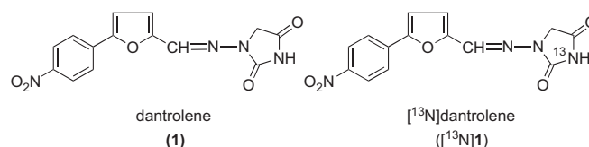
Scheme 1. Chemical structures of dantrolene ( 1 ) and [ ^{13}\text{N} ]dantrolene ([ ^{13}\text{N} ] 1 ).
